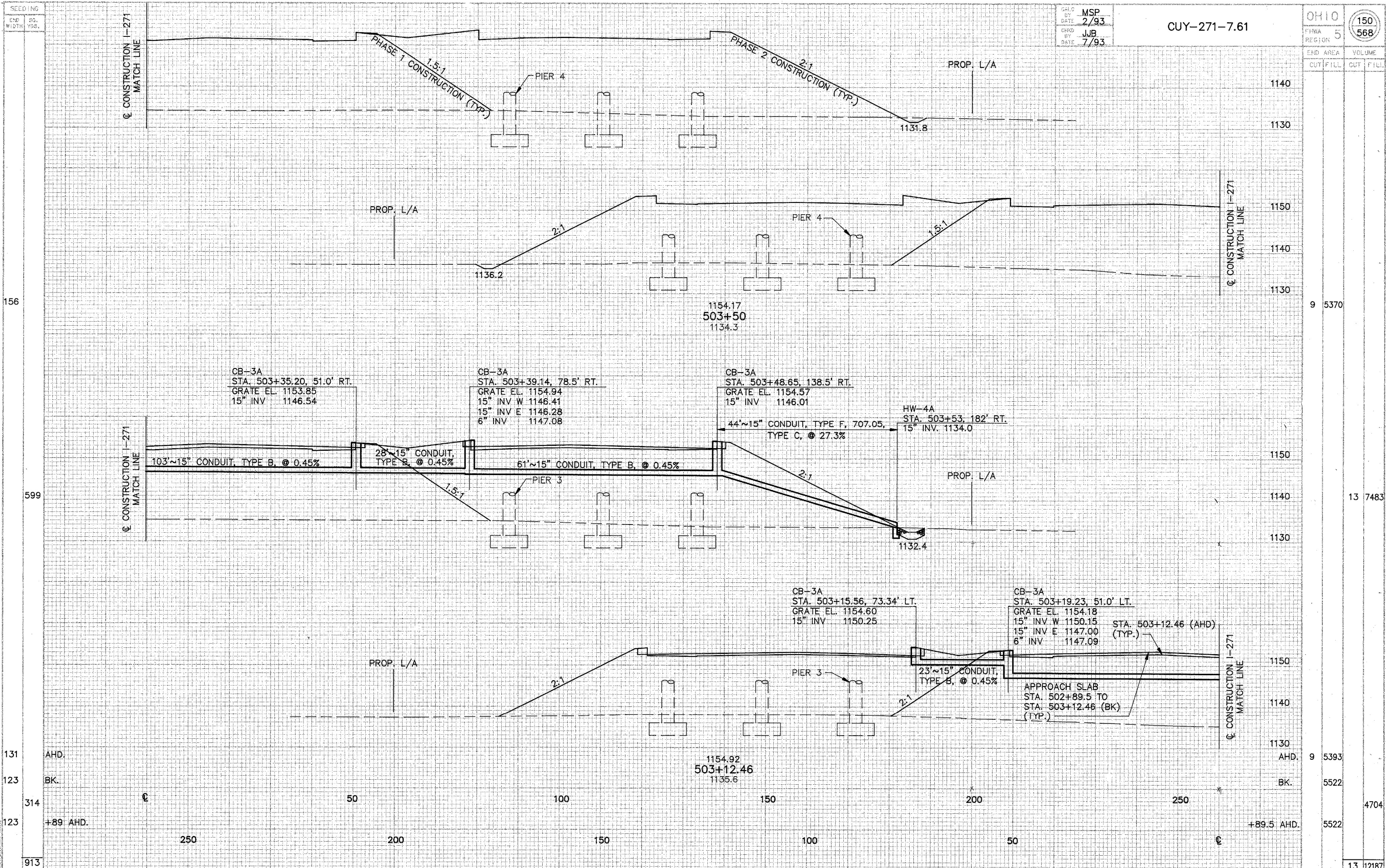
CROSS SECTIONS STA. 503+12.46 TO STA. 503+50
