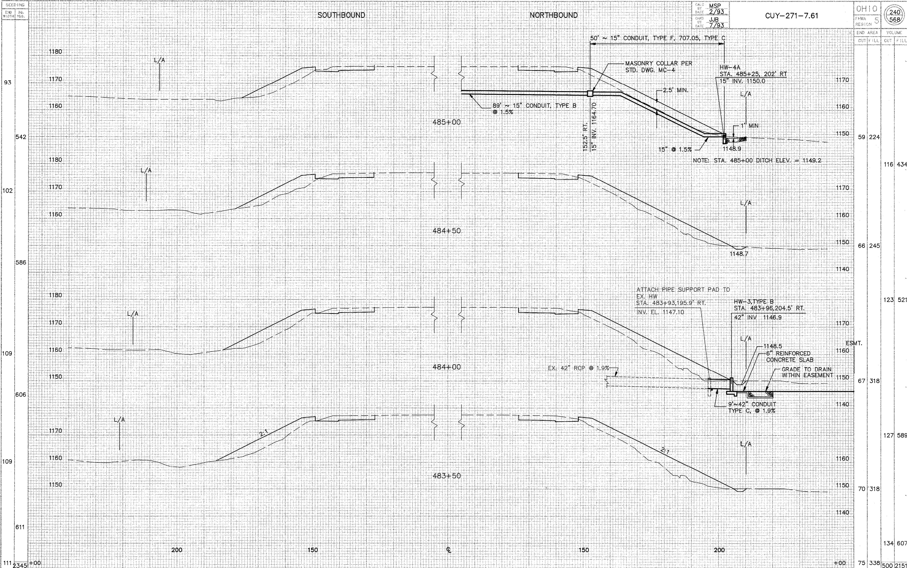
MAINLINE WIDENING CROSS SECTIONS STA. 483+50 TO STA. 485+00
