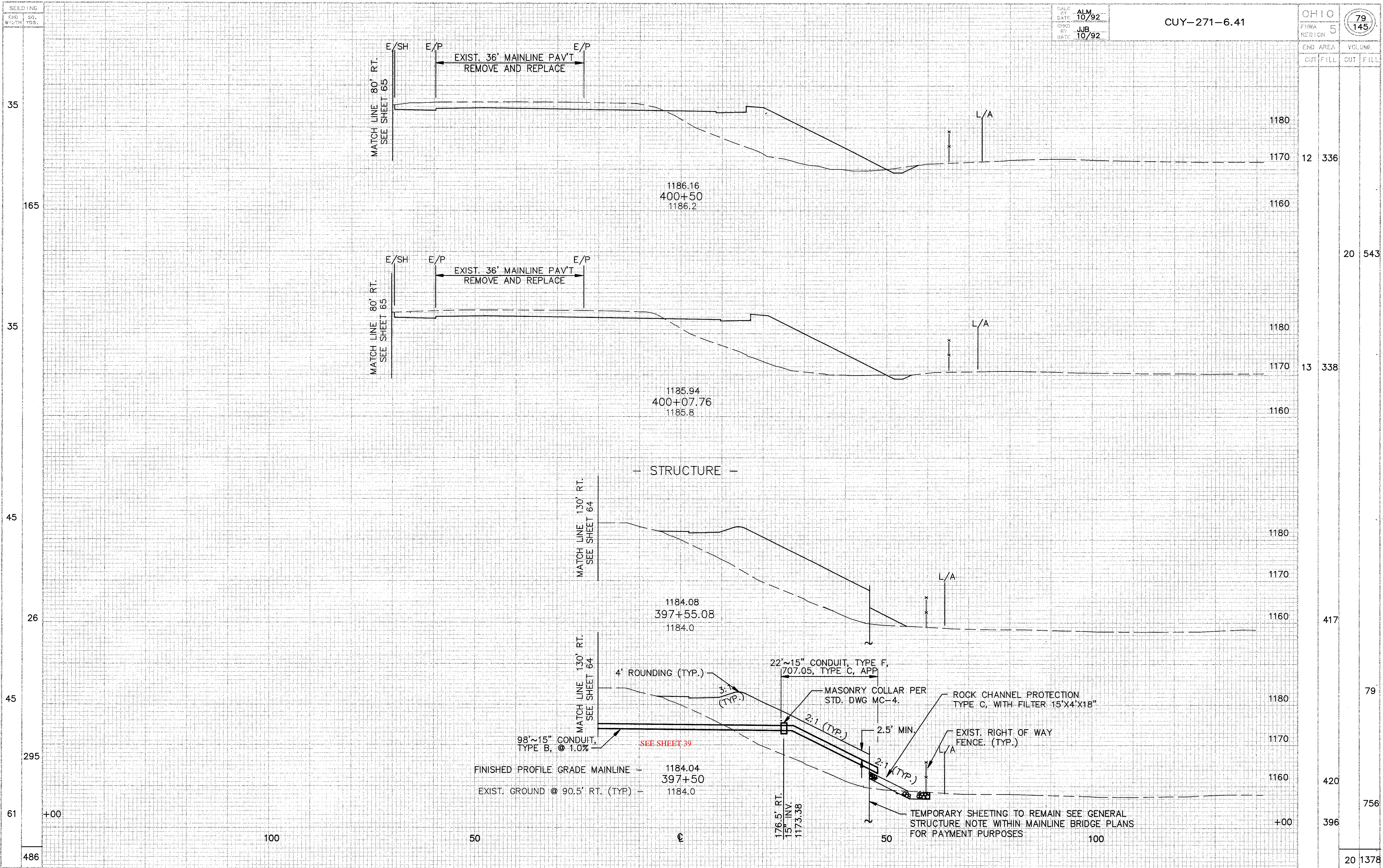
MAINLINE WIDENING CROSS SECTIONS STA. 397+50 TO STA. 400+50
