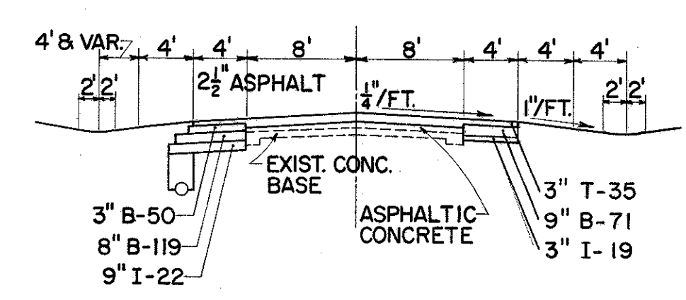
TYPICAL SECTION EXIST. BAGLEY ROAD
