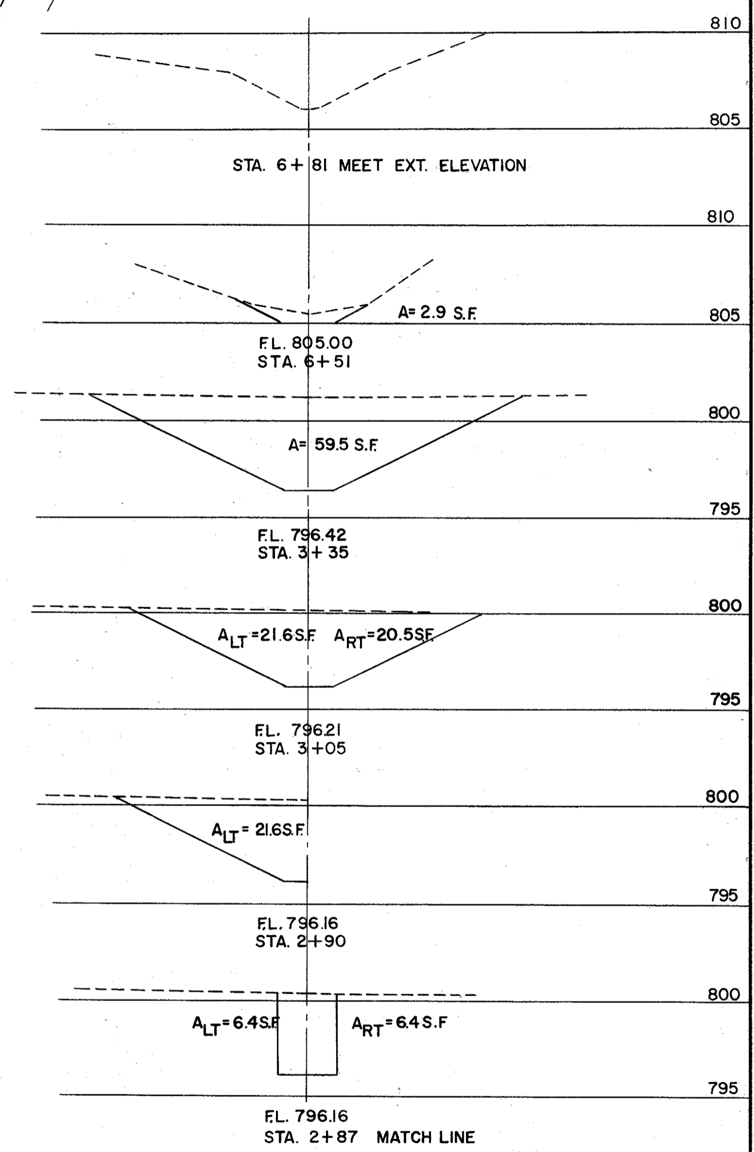
CHANNEL CROSS SECTIONS SCALE 1"=5'
