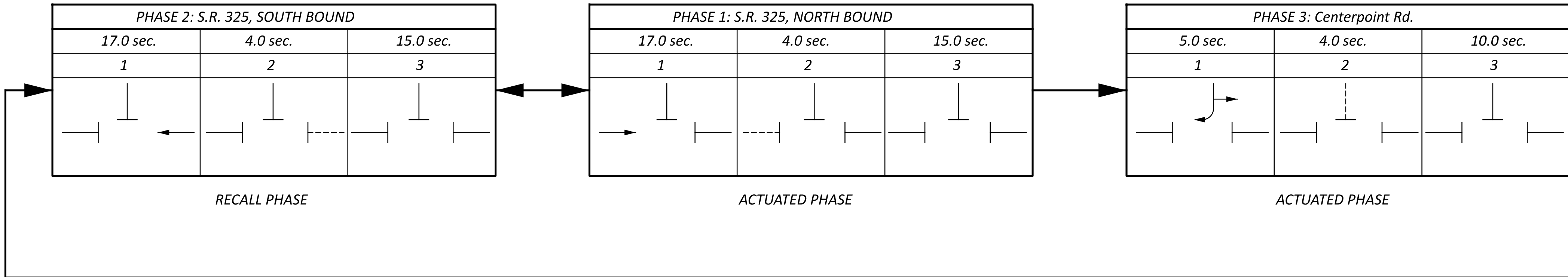
PHASE 1 - SIGNAL TIMING DIAGRAM
