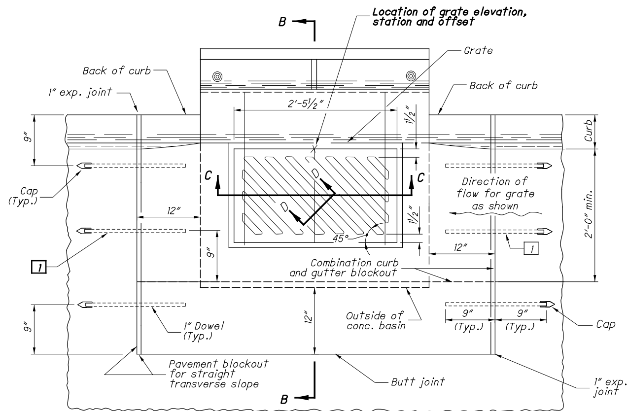
PLAN OF CATCH BASIN AND PAVEMENT JOINTS (For SECTIONS C-C and D-D, see Sht. 2/2)
