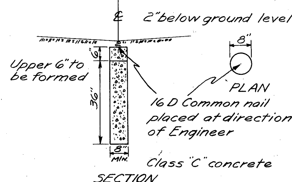
Detail of Centerline Reference Monuments
