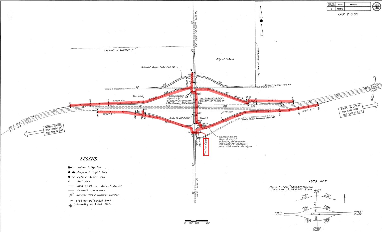
SCHEMATIC LAYOUT - LIGHTING CIRCUITS
