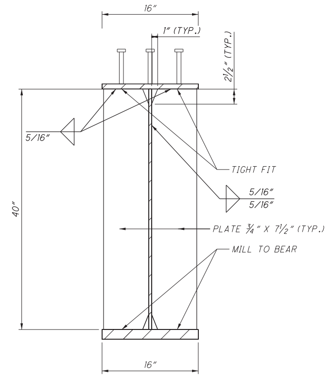
BEARING STIFFENERS FWD. & REAR ABUT. AT BEARING OF ALL GIRDERS
