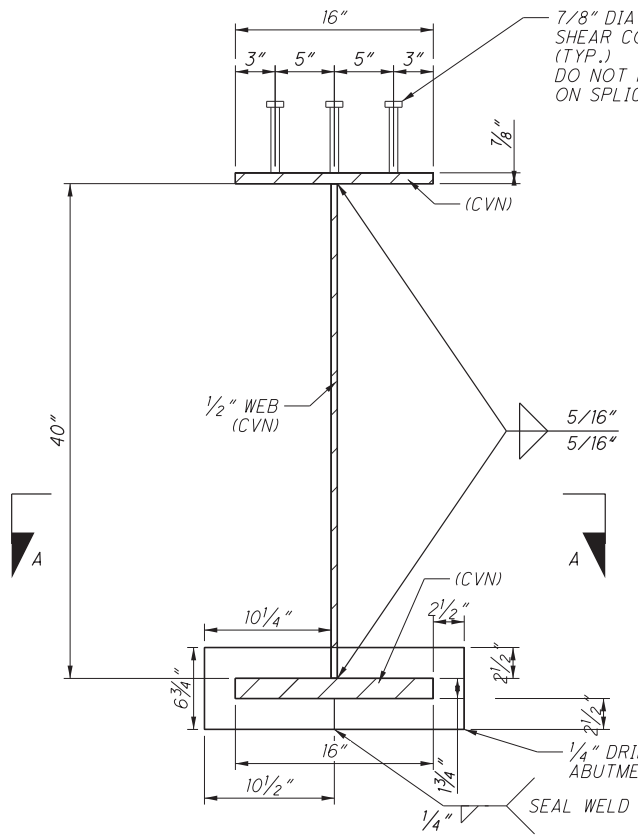
GIRDER AND SHEAR CONNECTOR DETAIL
