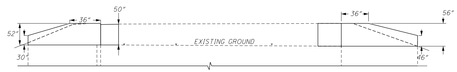
REAR ABUTMENT SEALANT DETAILS
