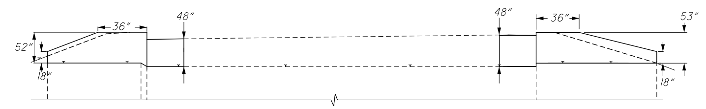
FORWARD ABUTMENT SEALANT DETAILS
