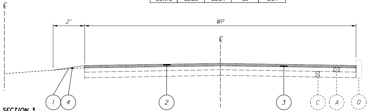
TYPICAL SECTION 3
