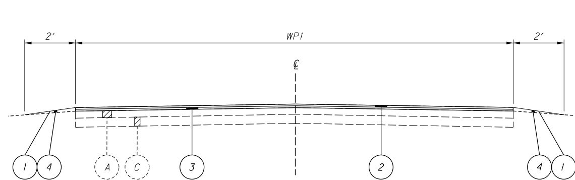
TYPICAL SECTION 2
