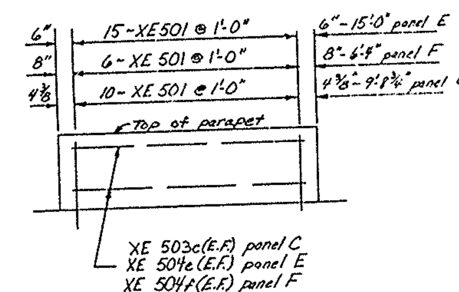
TYPICAL PARAPET SPACING
