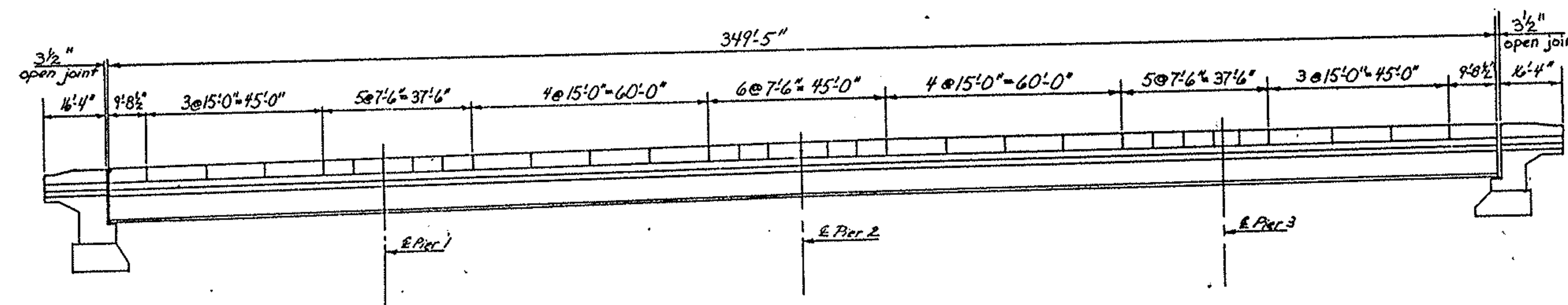
PROPOSED ELEVATION
