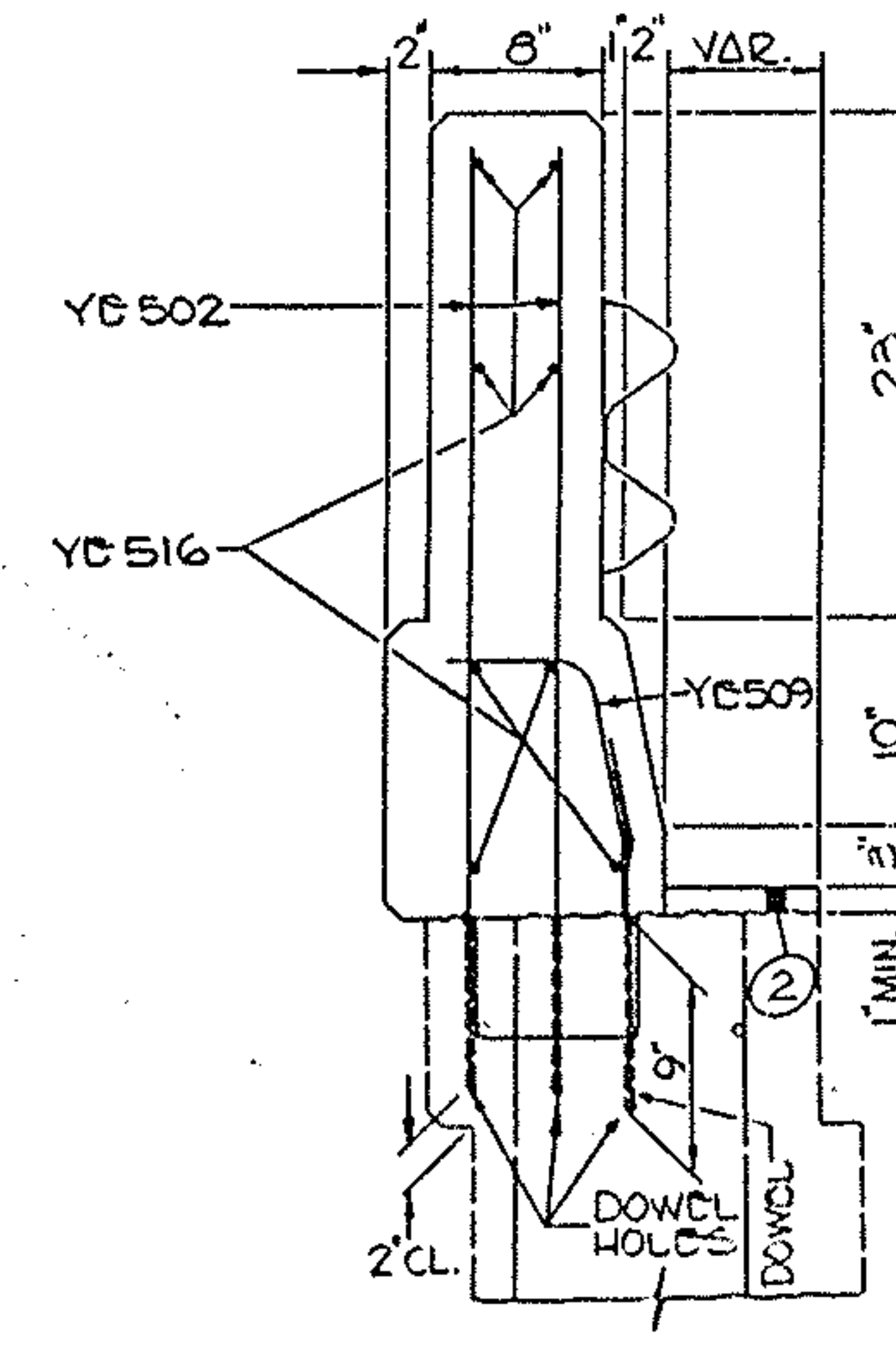
PROPOSED SECTION C-C
