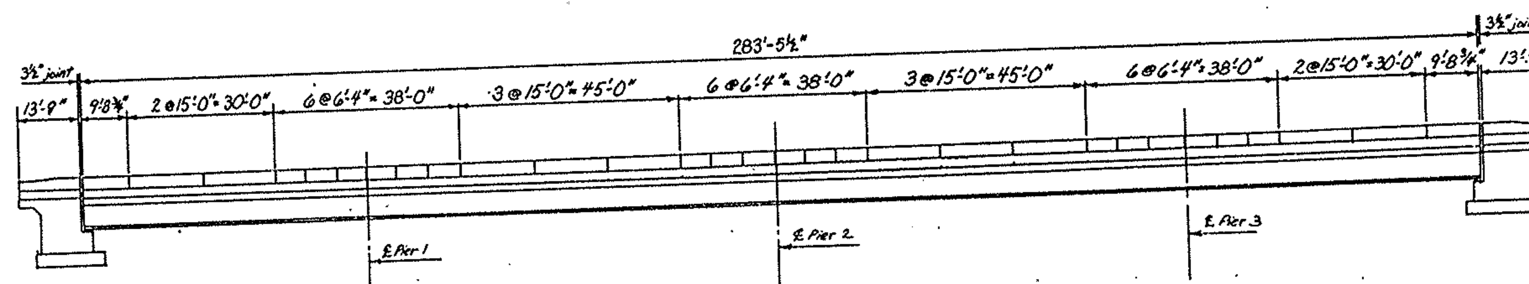
PROPOSED ELEVATION
