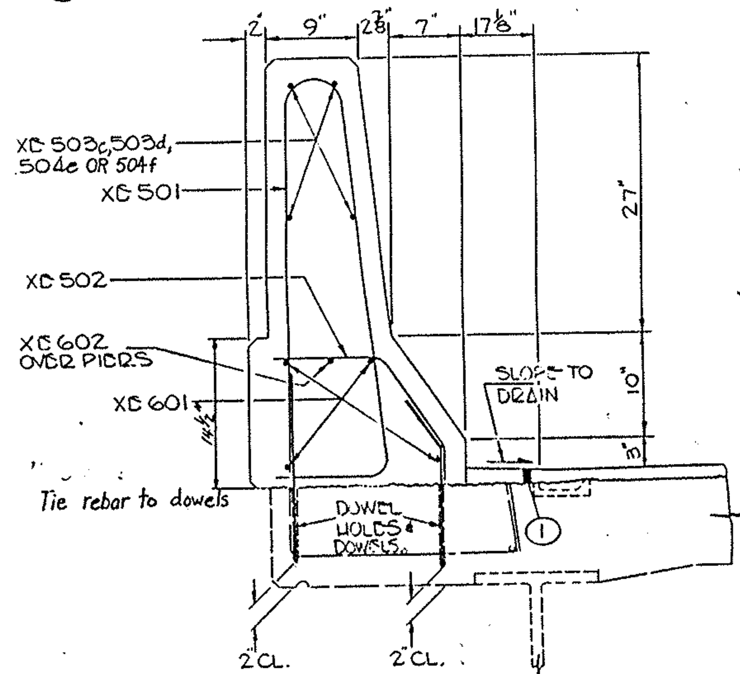
PROPOSED SECTION A-A
