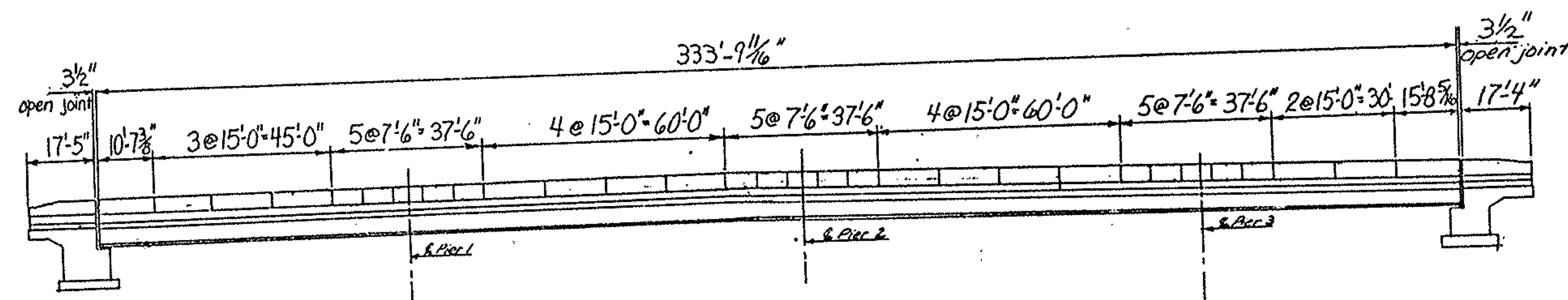
PROPOSED ELEVATION
