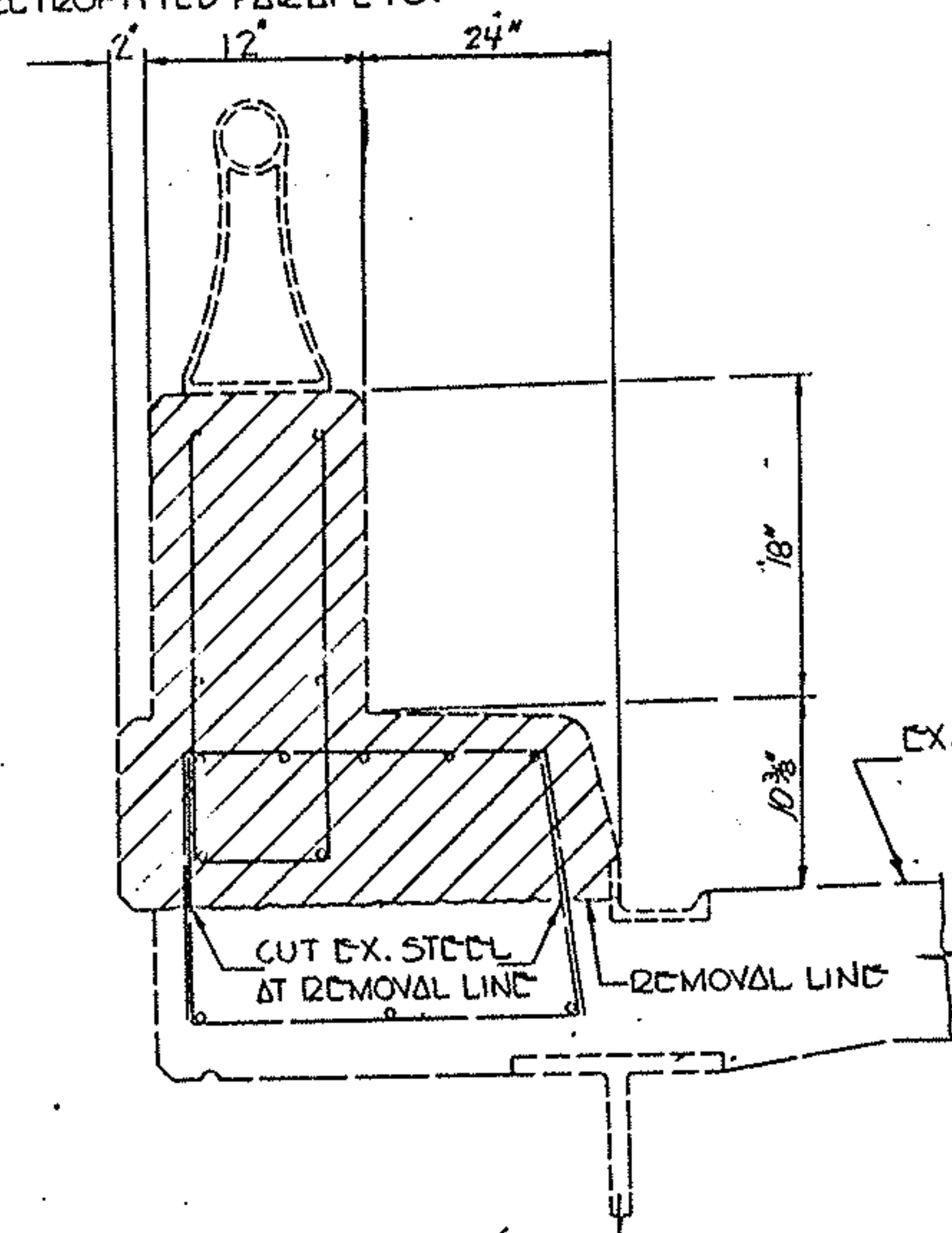
EXISTING SECTION A-A
