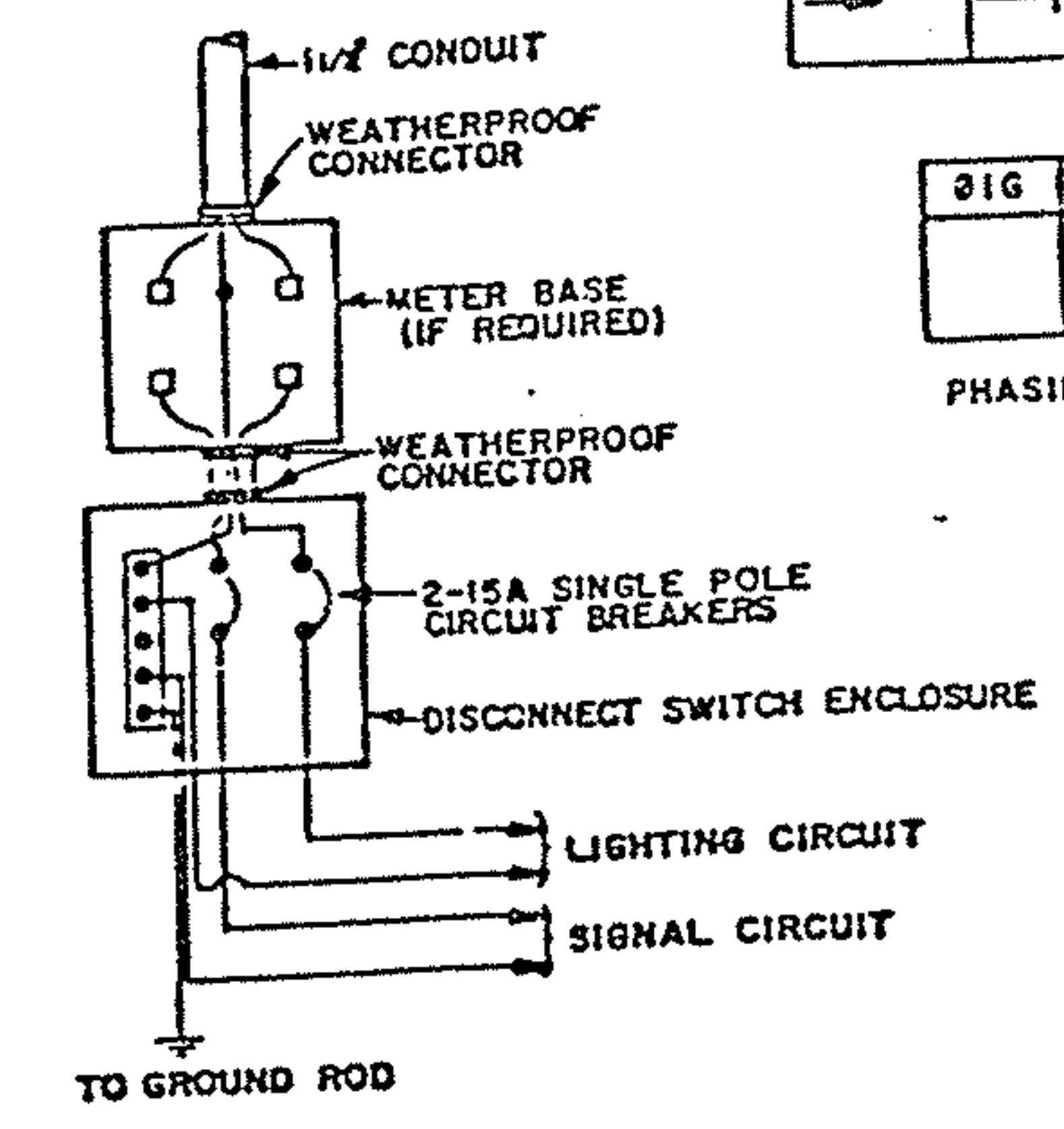
DETAIL "A"
