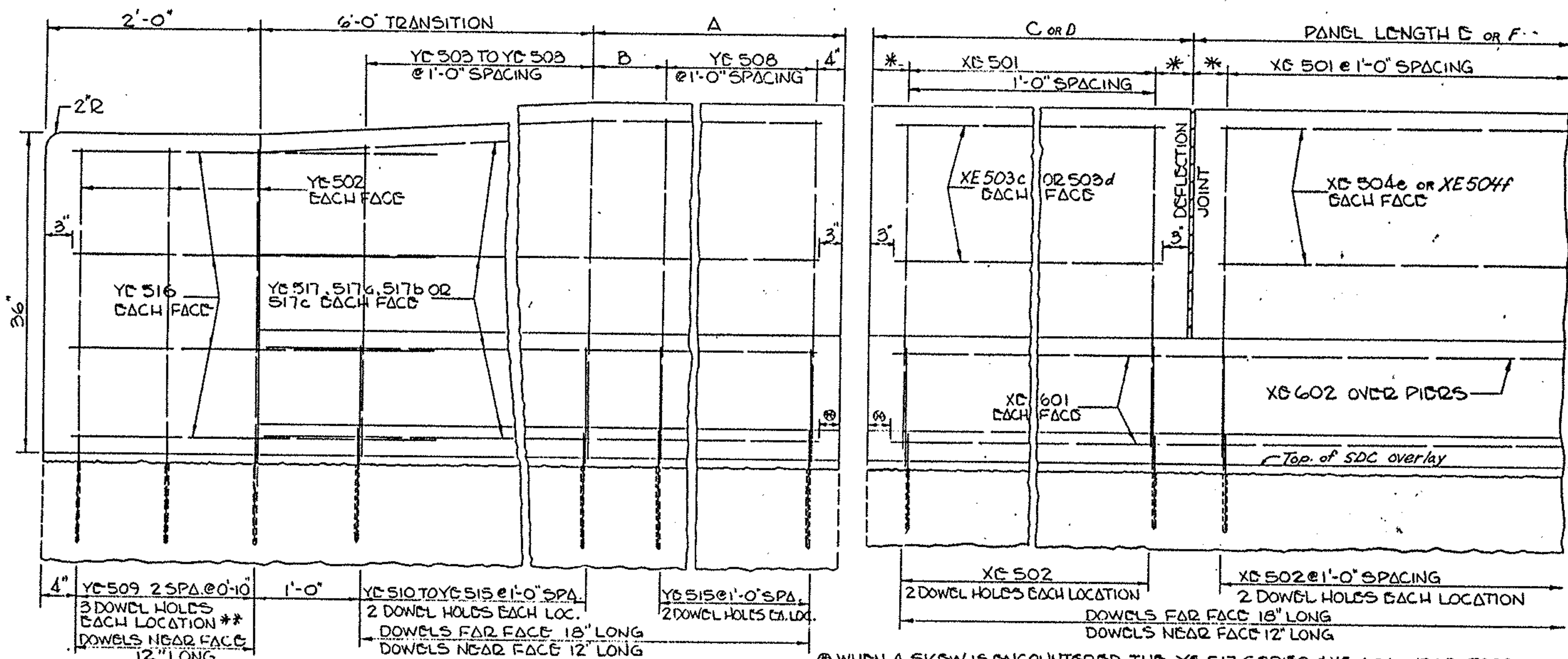
PROFILE VIEW
