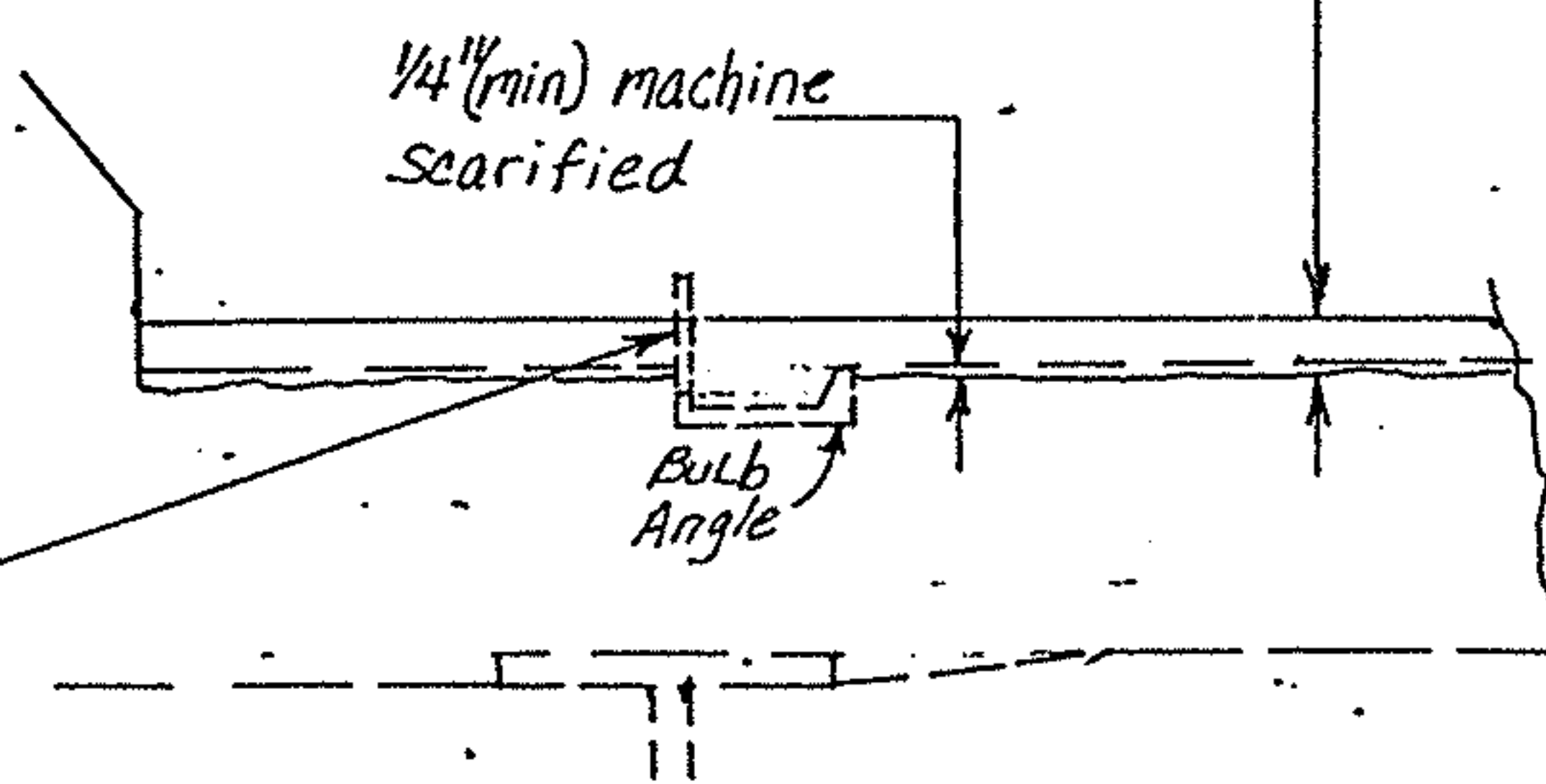
TYPICAL OVERLAY DETAIL AT BULB ANGLES
