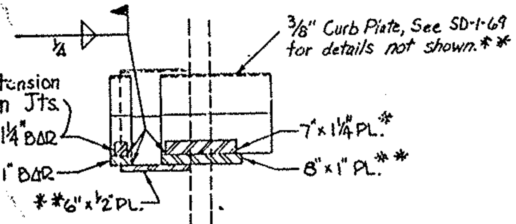
PROPOSED SECTION E-E
