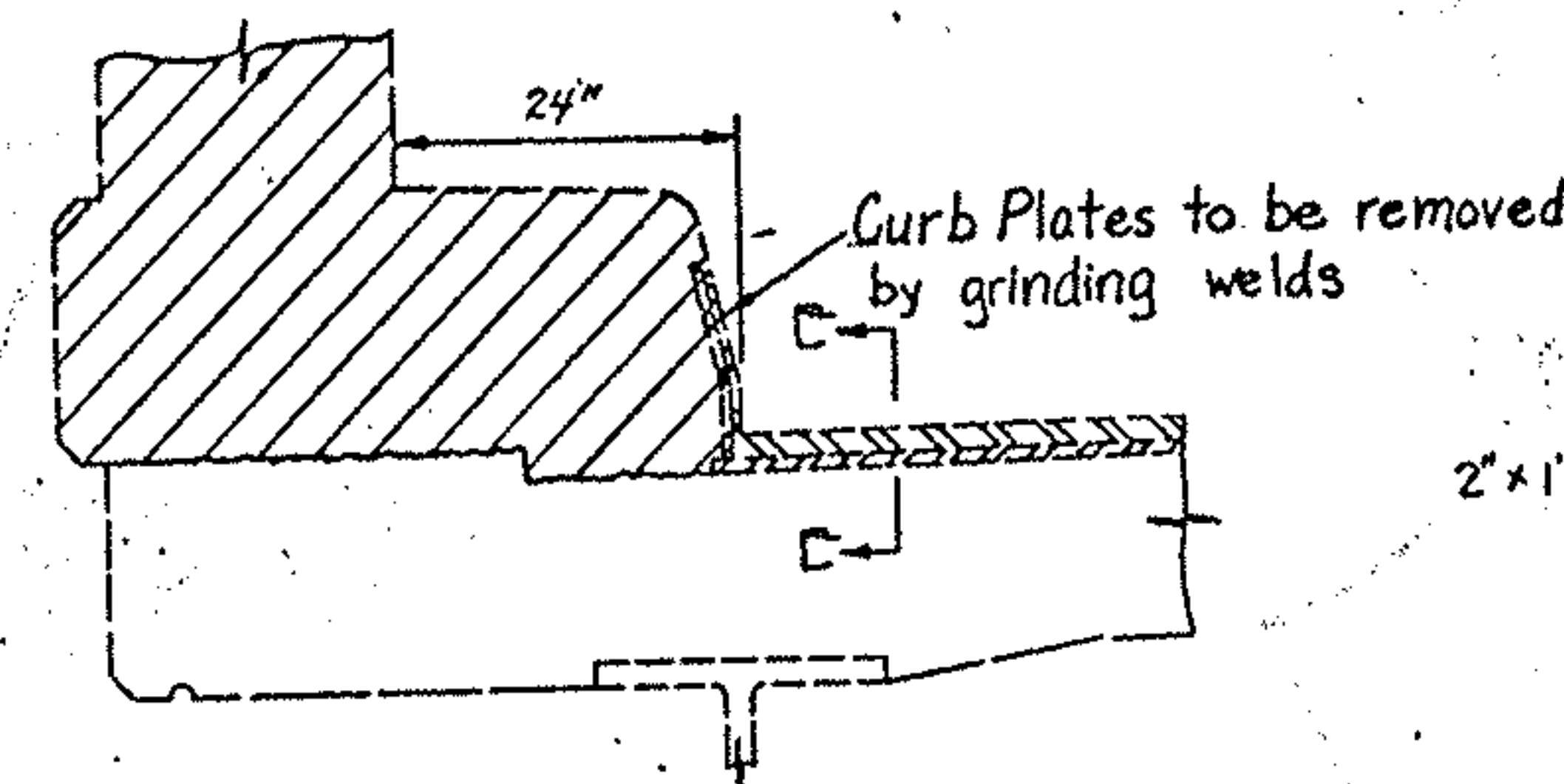
EXISTING SECTION D-D
