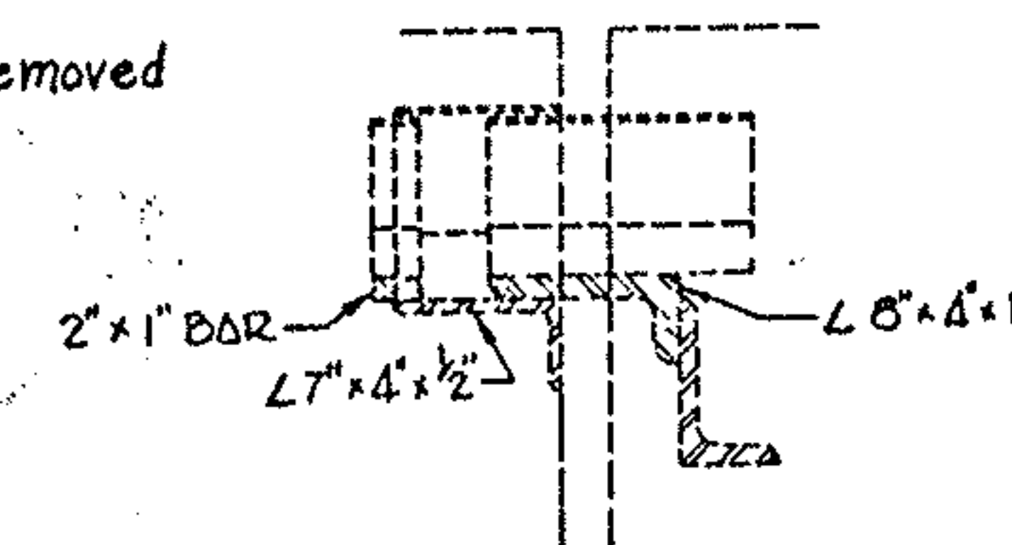
EXISTING SECTION E-E
