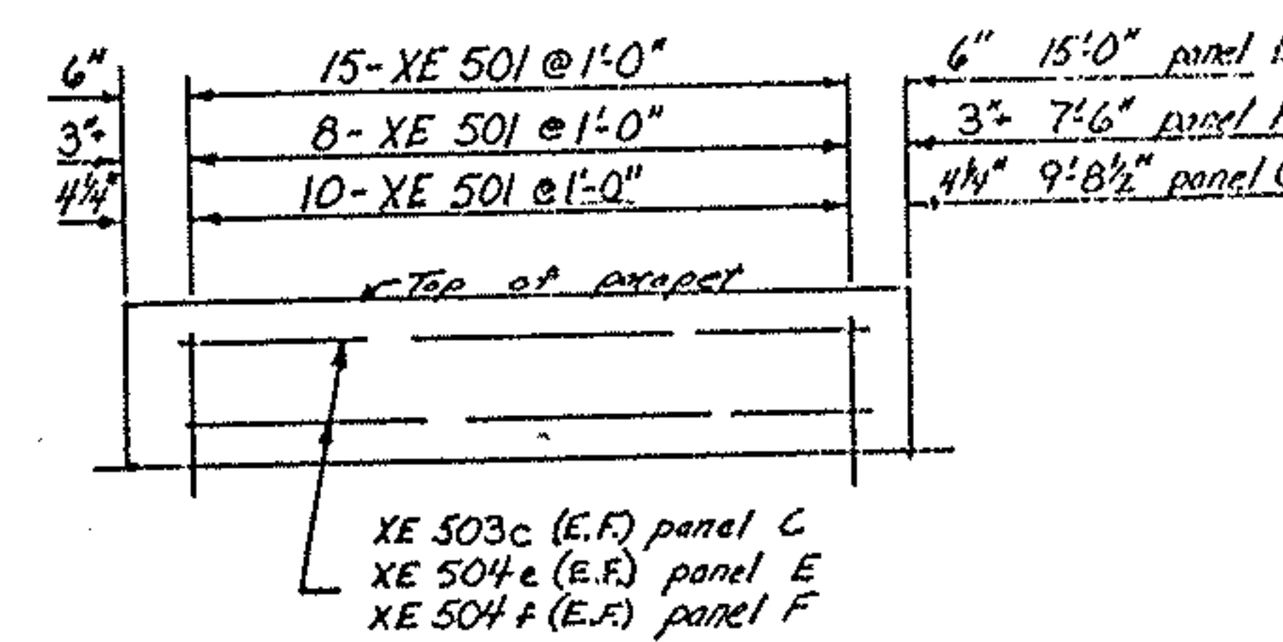
TYPICAL PARAPET SPACING
