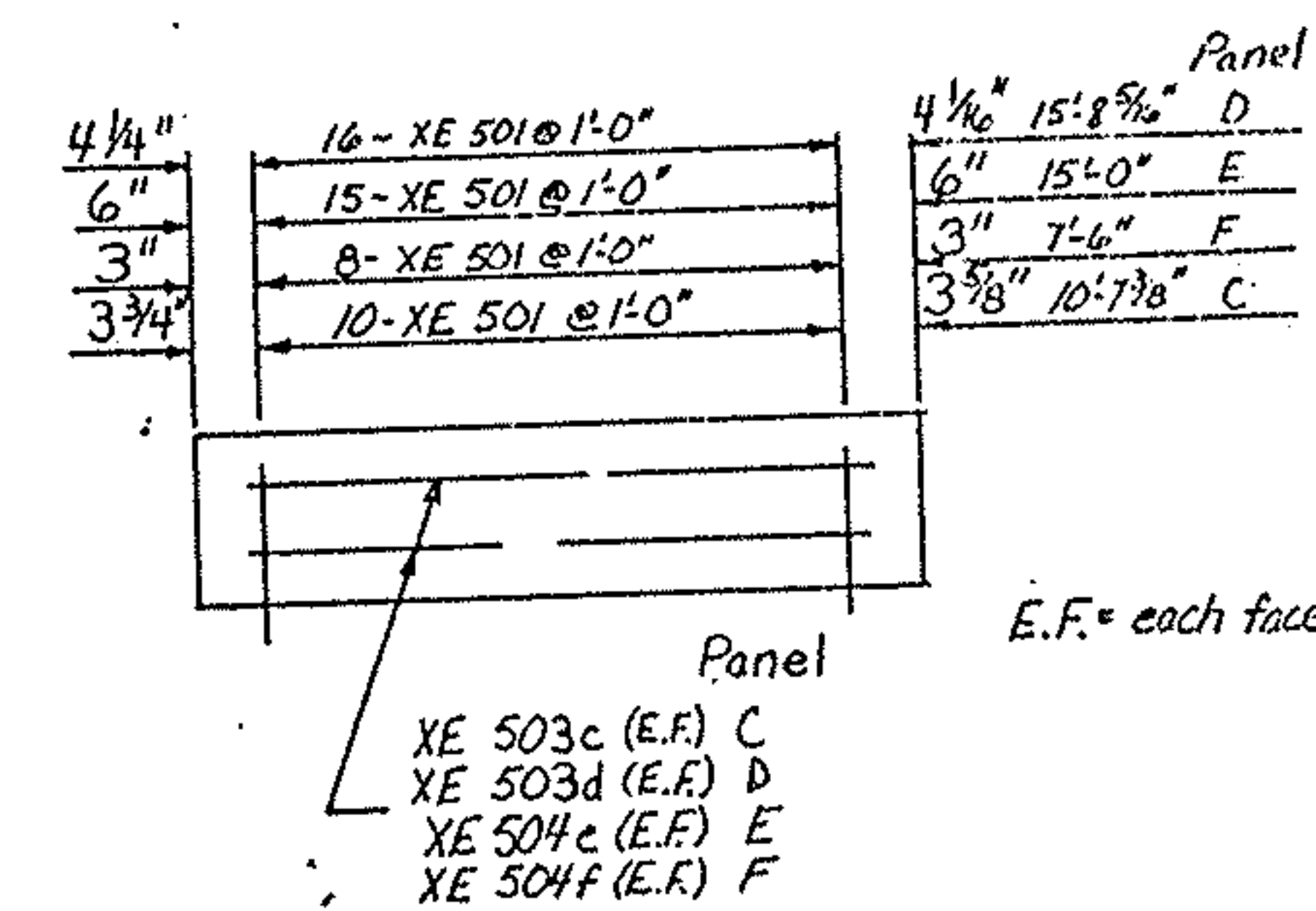
TYPICAL PARAPET SPACING
