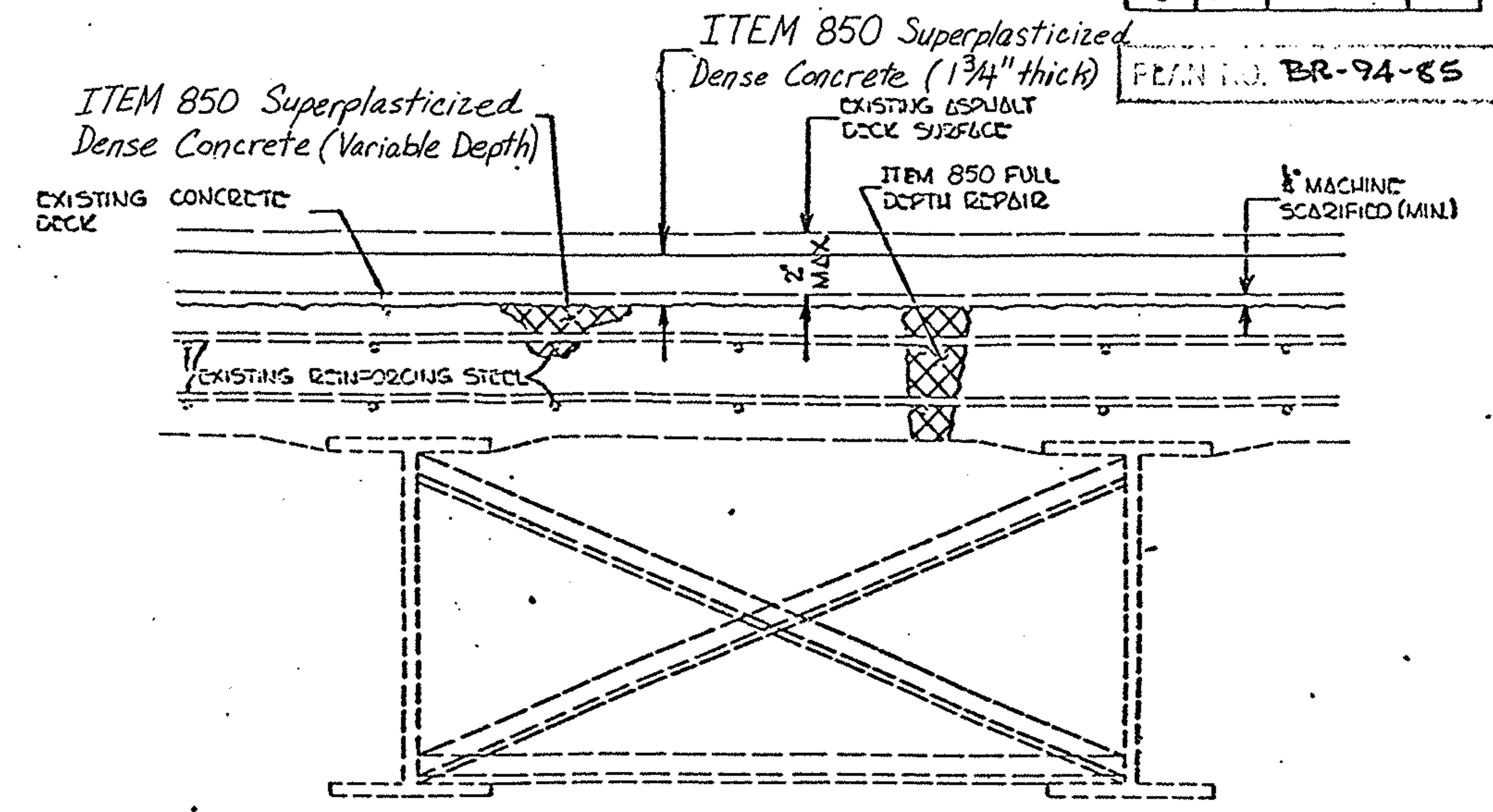
SUPERPLASTICIZED DENSE CONCRETE OVERLAY
