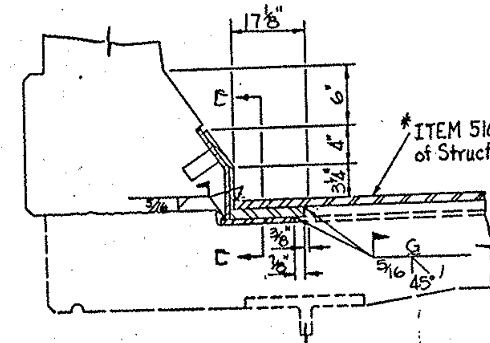
PROPOSED SECTION D-D
