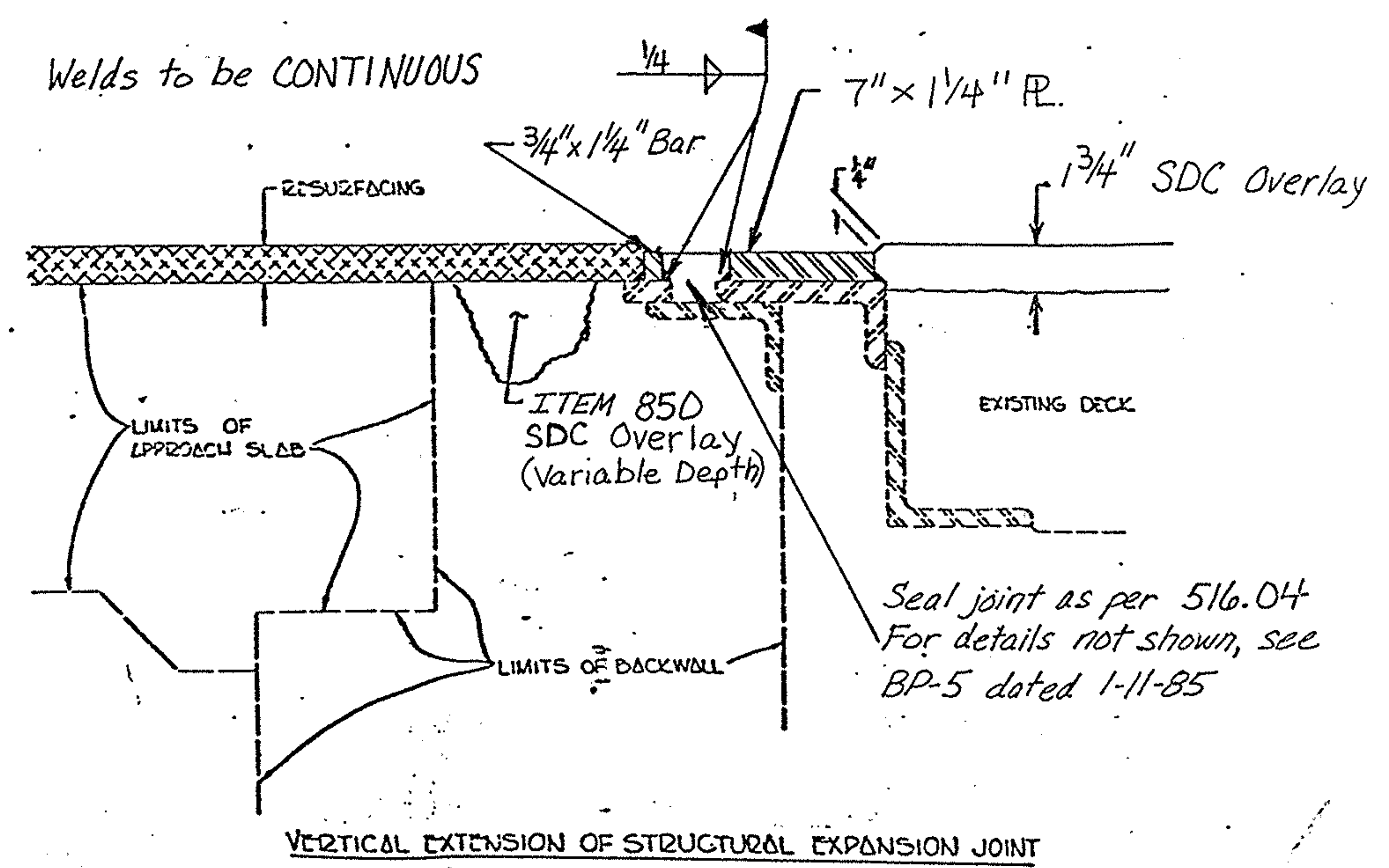
SUPERPLASTICIZED DENSE CONCRETE OVERLAY
