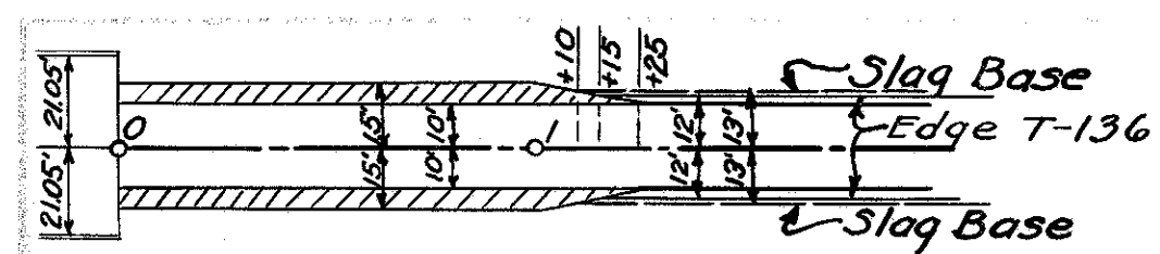
DETAIL of TRANSITION
