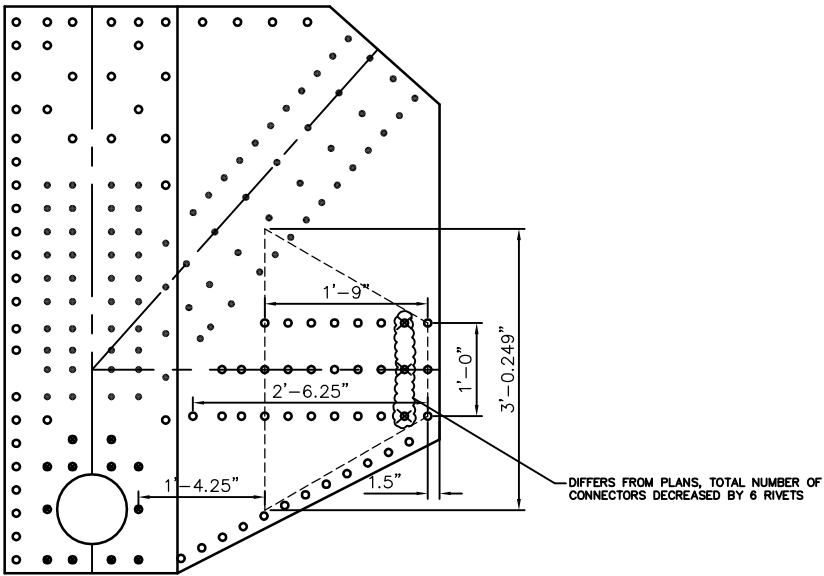
LOWER CHORD DIMENSIONS
