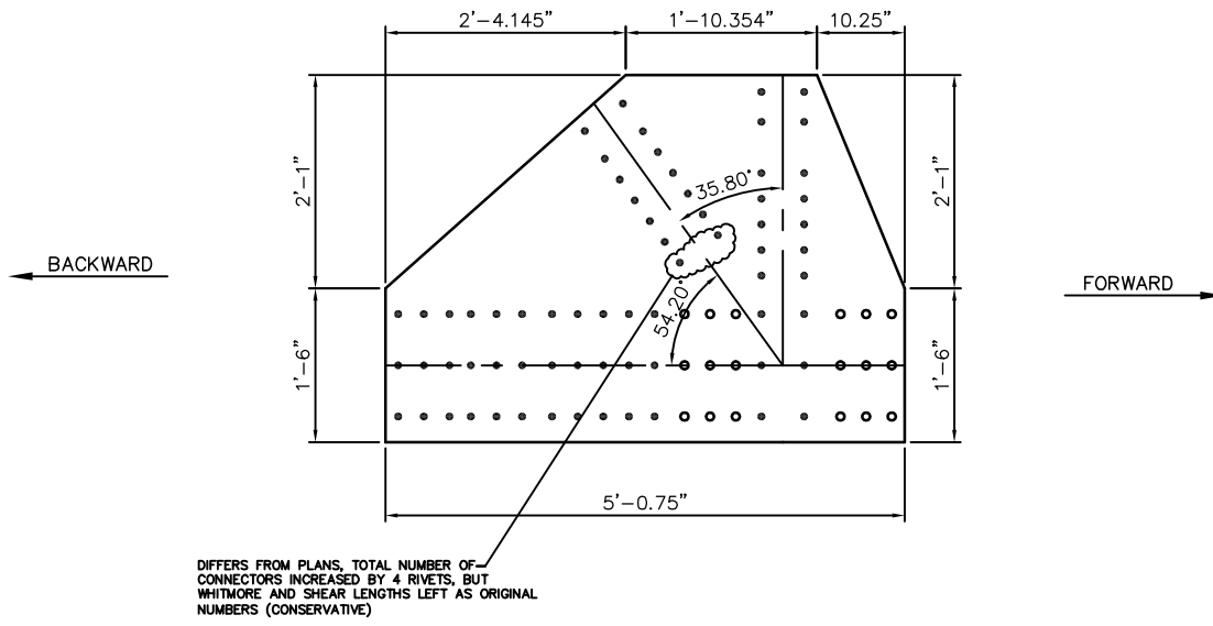
GENERAL GUSSET PLATE DIMENSIONS
