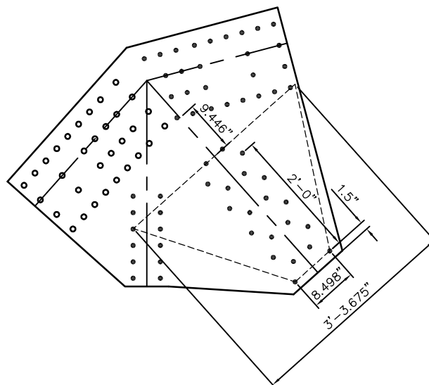
DIAGONAL DIMENSIONS
