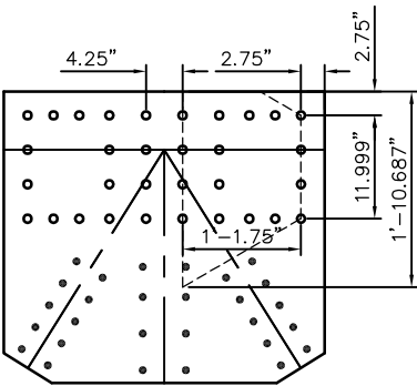
UPPER CHORD DIMENSIONS
