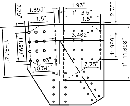
UPPER CHORD DIMENSIONS
