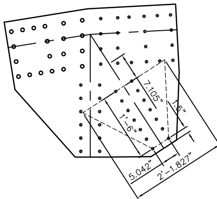
DIAGONAL DIMENSIONS
