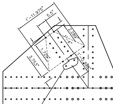
DIAGONAL DIMENSIONS
