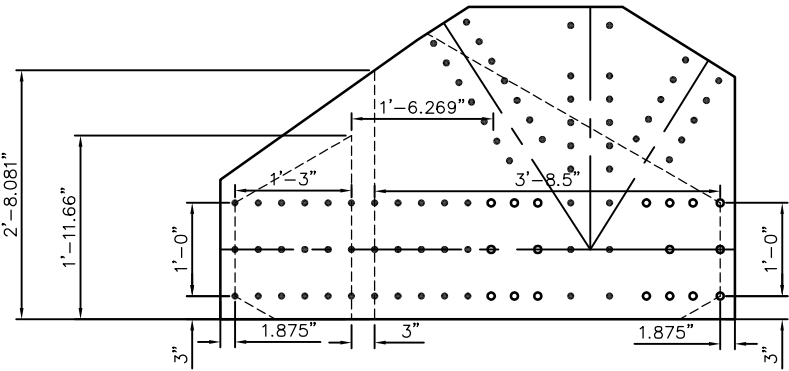
LOWER CHORD DIMENSIONS
