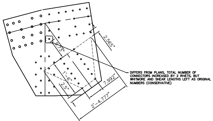
DIAGONAL DIMENSIONS
