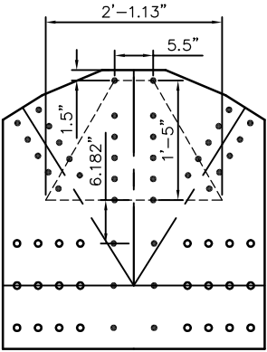
VERTICAL DIMENSIONS
