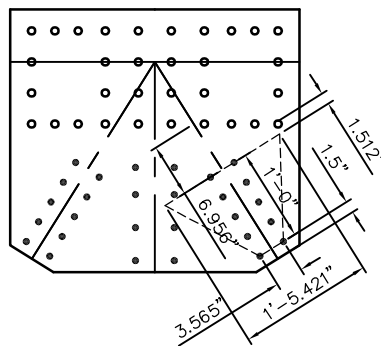
DIAGONAL DIMENSIONS
