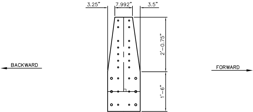
GENERAL GUSSET PLATE DIMENSIONS
