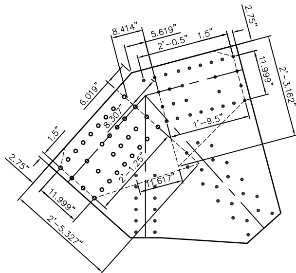
UPPER CHORD DIMENSIONS
