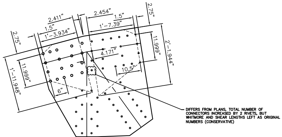
UPPER CHORD DIMENSIONS
