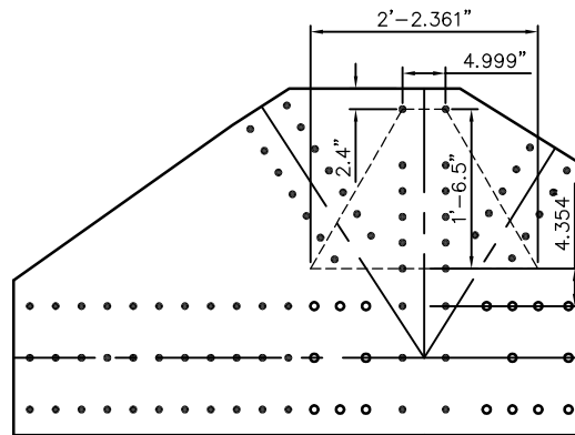
VERTICAL DIMENSIONS
