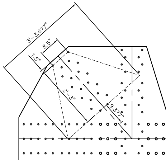
DIAGONAL DIMENSIONS
