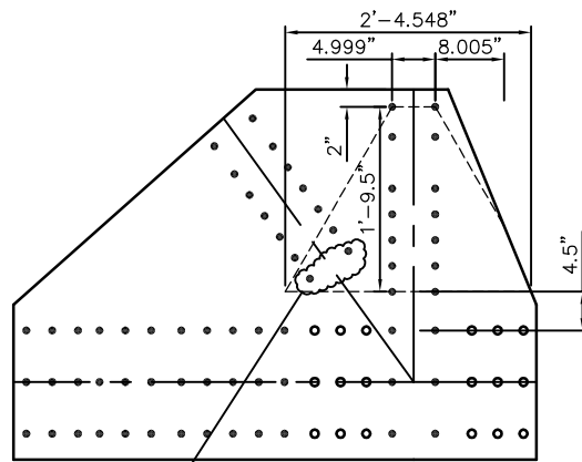
VERTICAL DIMENSIONS
