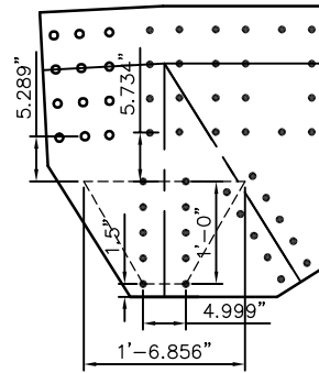
VERTICAL DIMENSIONS
