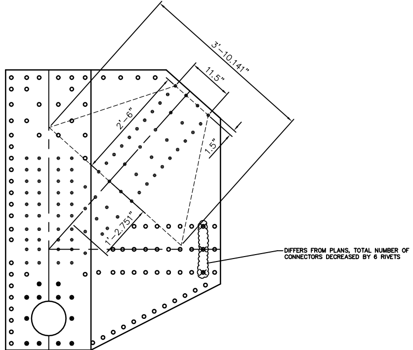
DIAGONAL DIMENSIONS
