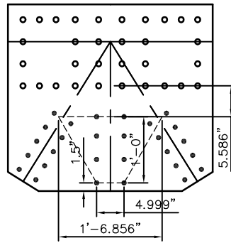
VERTICAL DIMENSIONS
