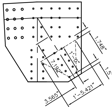
DIAGONAL DIMENSIONS
