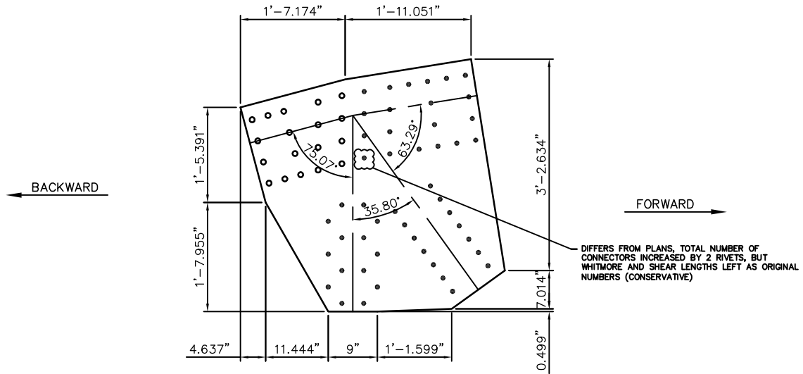
GENERAL GUSSET PLATE DIMENSIONS
