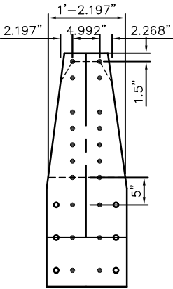
LOWER CHORD DIMENSIONS
