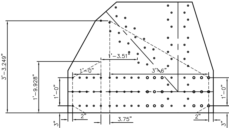
LOWER CHORD DIMENSIONS
