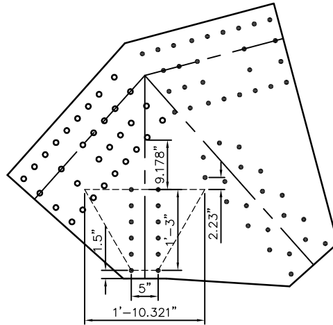
VERTICAL DIMENSIONS
