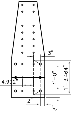
LOWER CHORD DIMENSIONS
