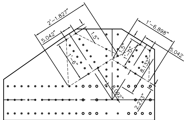
DIAGONAL DIMENSIONS
