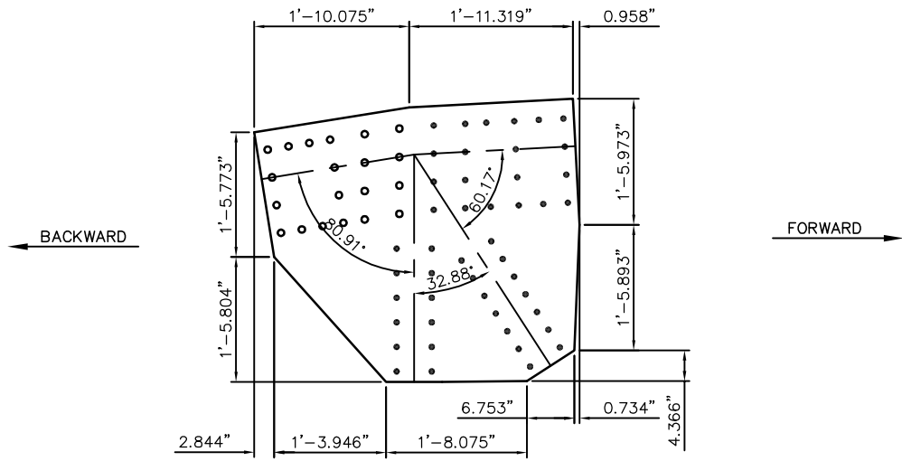
GENERAL GUSSET PLATE DIMENSIONS
