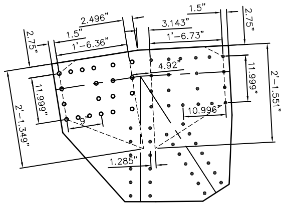
UPPER CHORD DIMENSIONS
