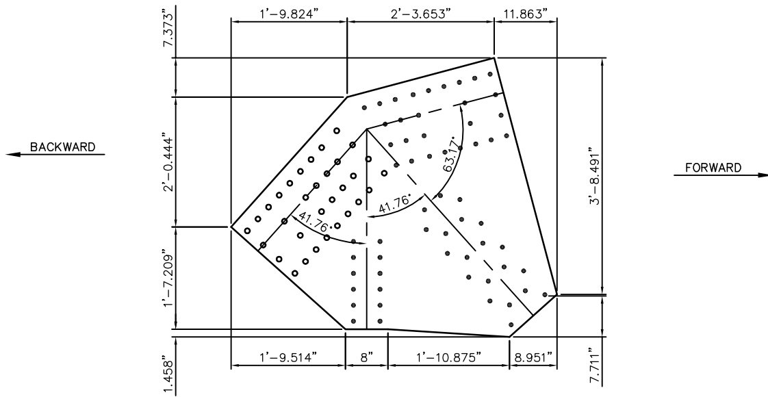
GENERAL GUSSET PLATE DIMENSIONS
