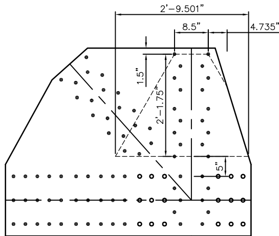
VERTICAL DIMENSIONS
