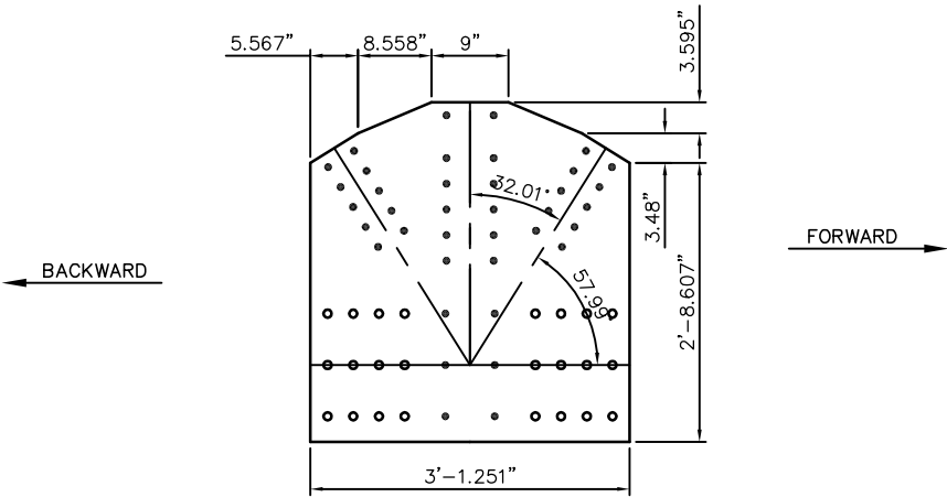
GENERAL GUSSET PLATE DIMENSIONS
