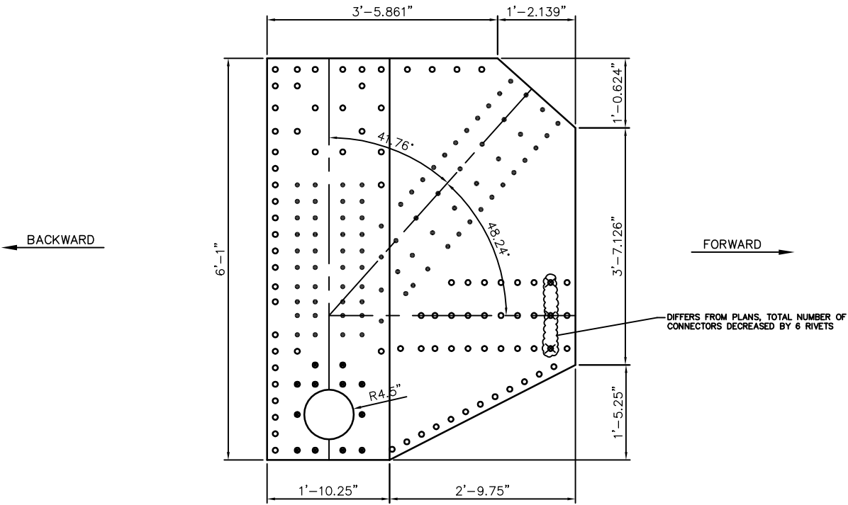
GENERAL GUSSET PLATE DIMENSIONS
