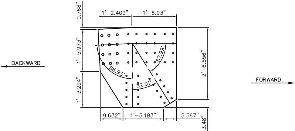
GENERAL GUSSET PLATE DIMENSIONS
